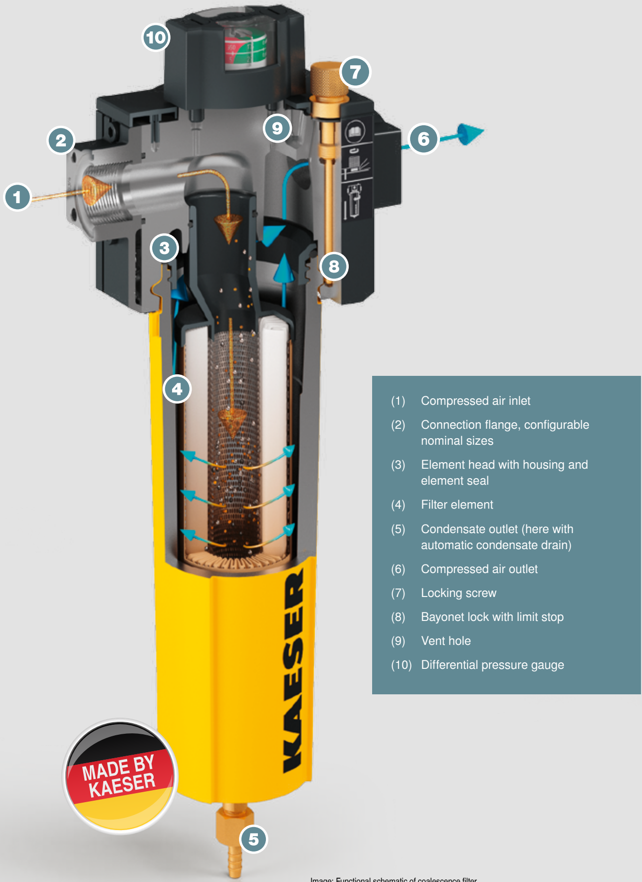
Image: Functional schematic of coalescence filter
